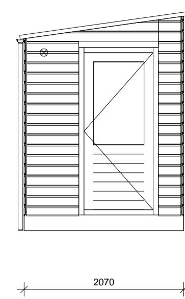
Dubbele berging hout - links
